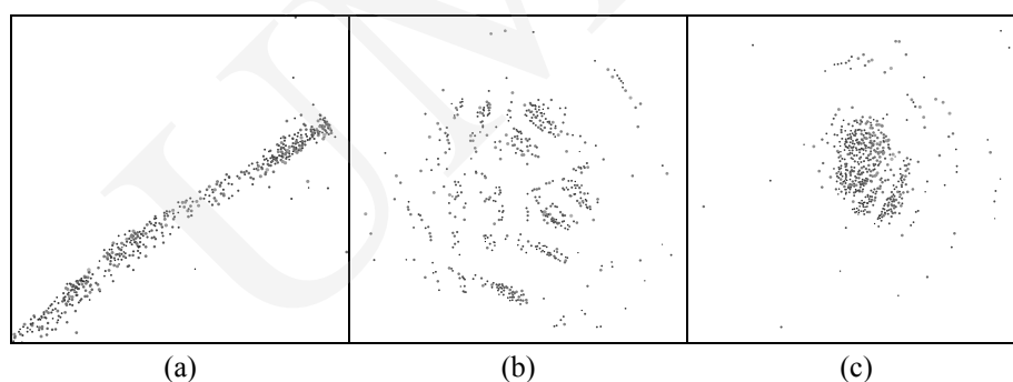
Fig. 2. The comparison of the normalization methods (data set cervix )
