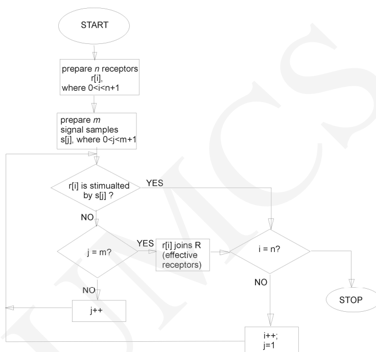
Fig 8. The algorithm of effective receptors set creation
