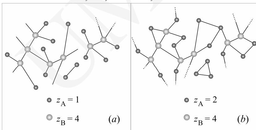
Fig. 1. Two schemes of binary alloy structures discussed in the paper for: (a) c_A = 0.65, c_B = 0.35 and z_A = 1, z_B = 4 , (b) c_A = 0.7, c_B = 0.3 and z_A = 2, z_B = 4 , respectively
