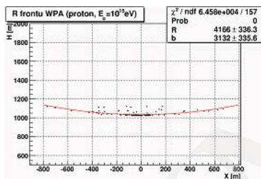
Fig. 8. An example illustrating a circle function fit conducted with ROOT.
