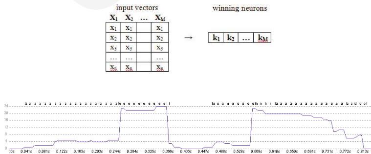
Fig. 3. Winning neuron contour of the utterance "ze gniazdo". Kohonen network size: 5x5.
